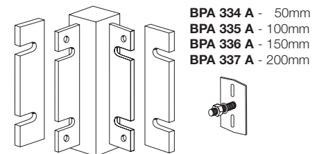
5 Axiom Profile Corner Post Kit
